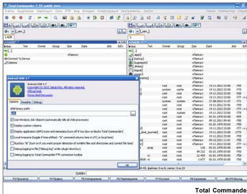
Total Commander
