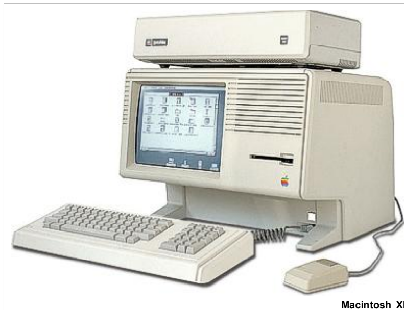
Macintosh XL
